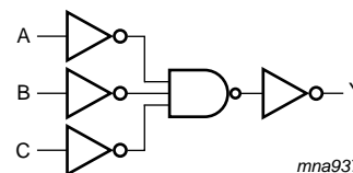
Fig 3. Logic diagram
